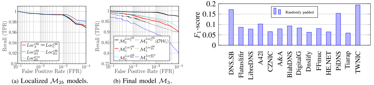
Figure A.5: Complete rundown of the recall values of the final and the localized models for considerably low FPR values.
